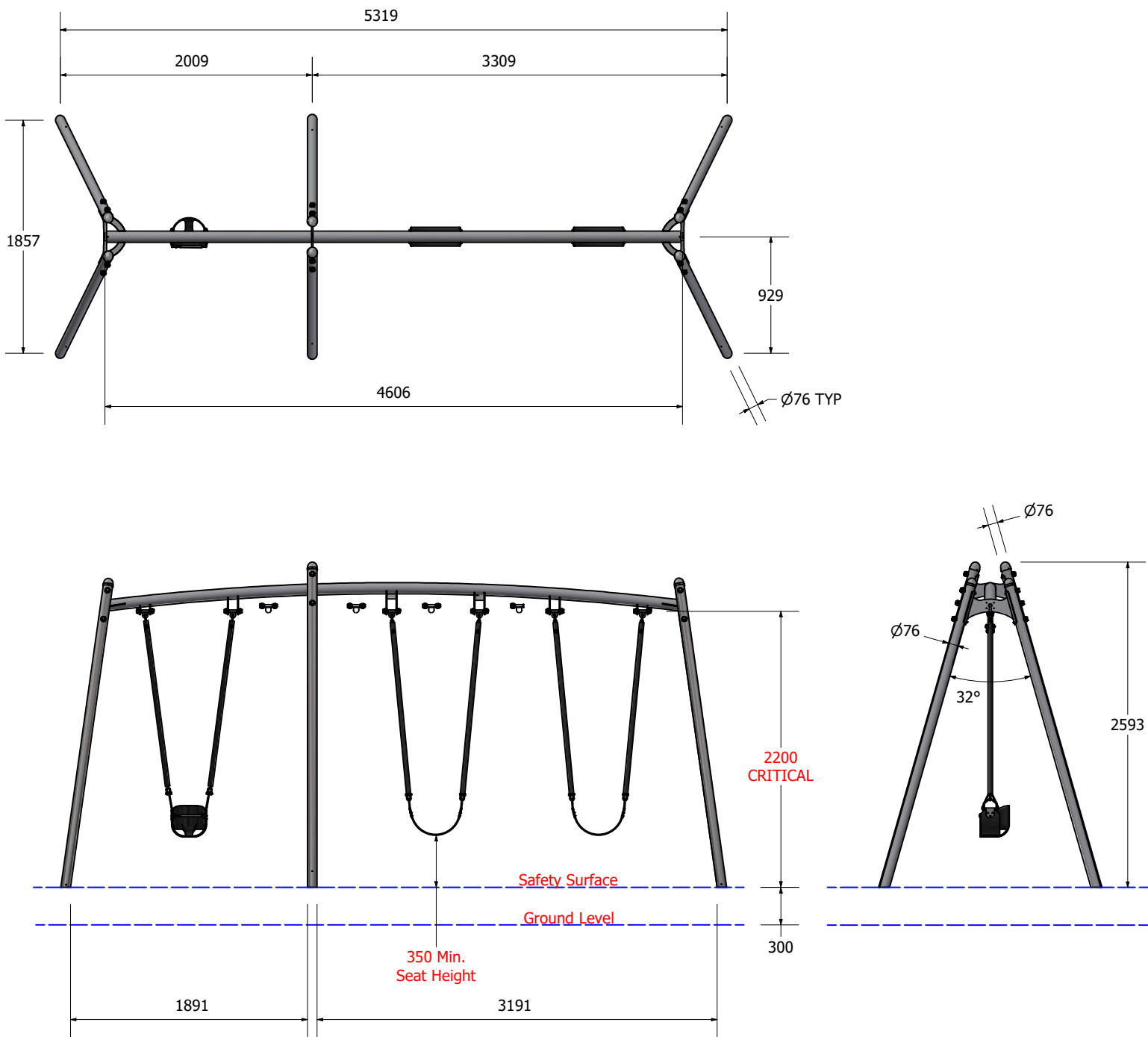
DIMENSIONS AT GROUND LEVEL
